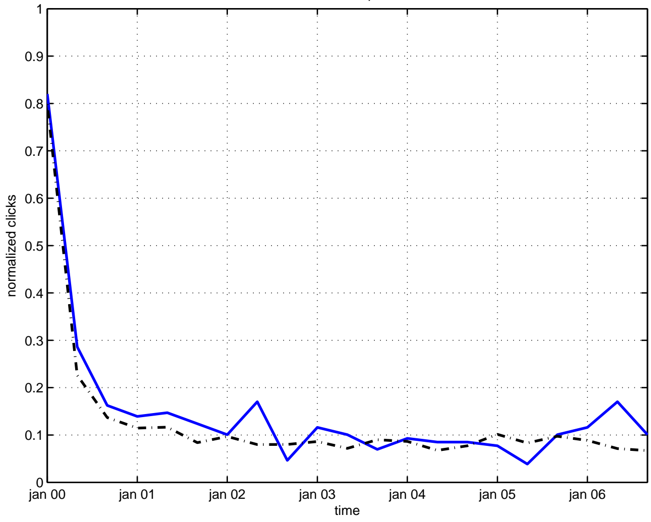
interaction quark
