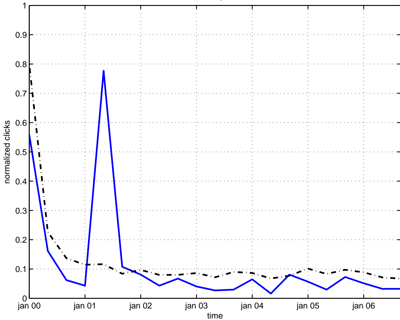
interaction p-brane
