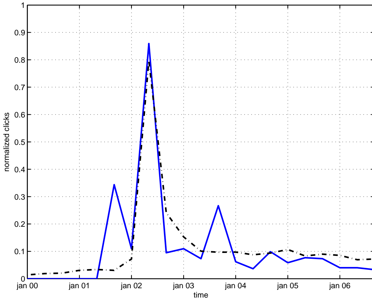
interaction oscillator
