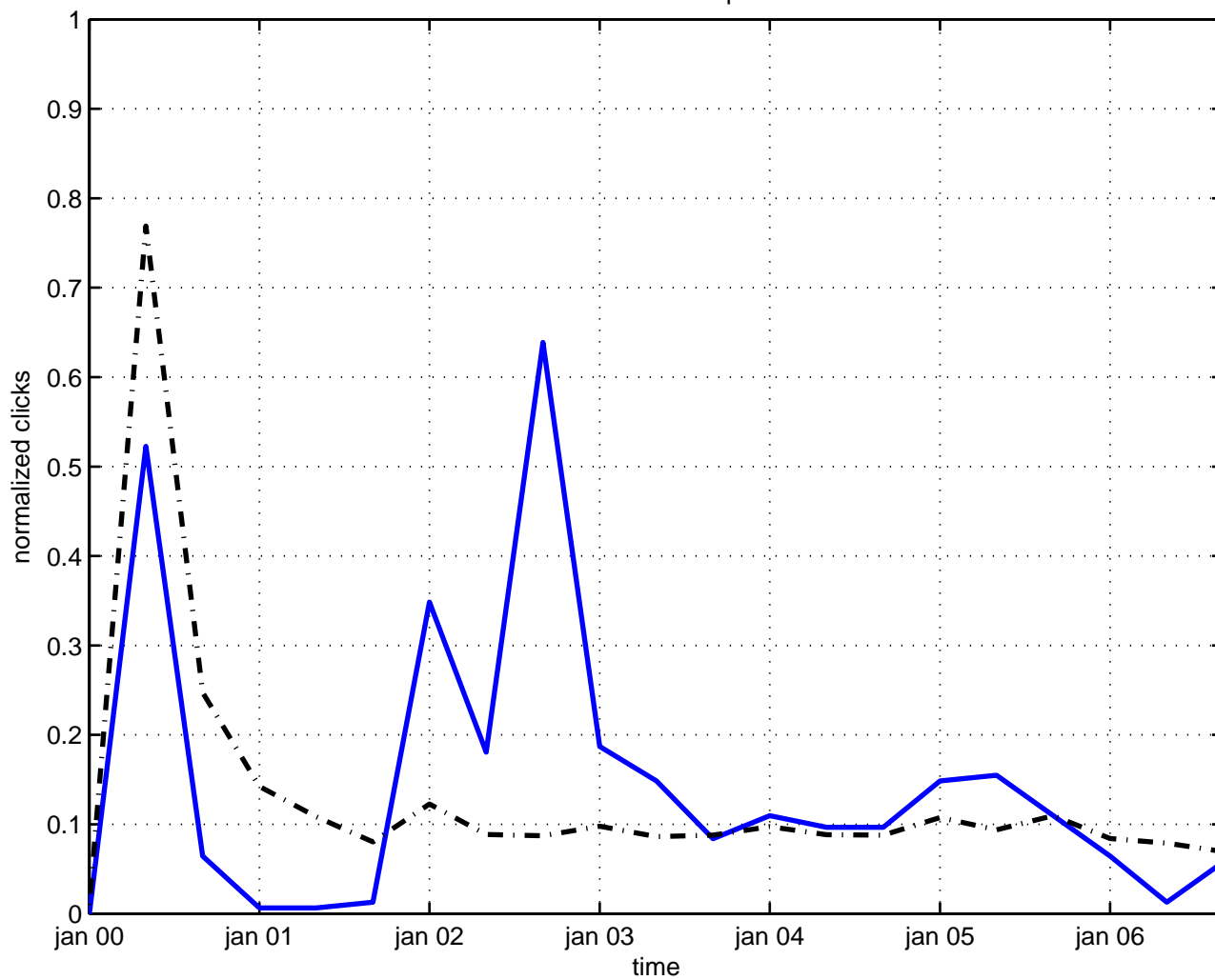
interaction monopole
