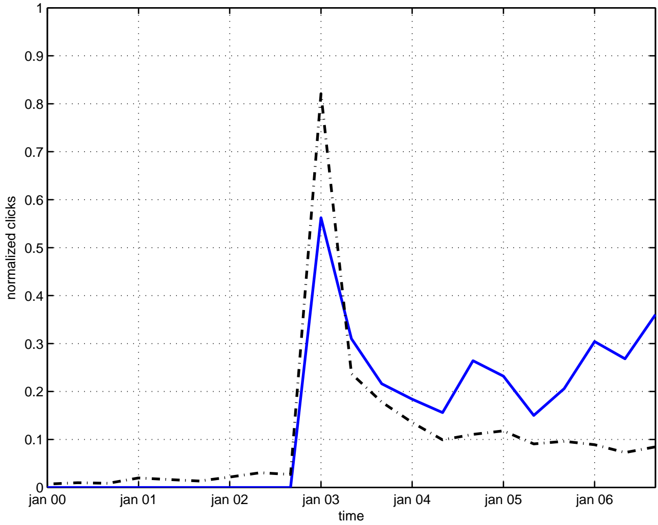
interaction meson
