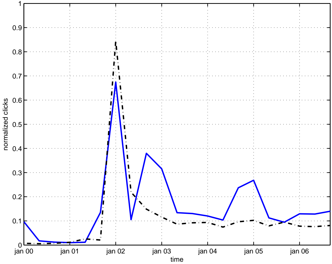
interaction field theory
