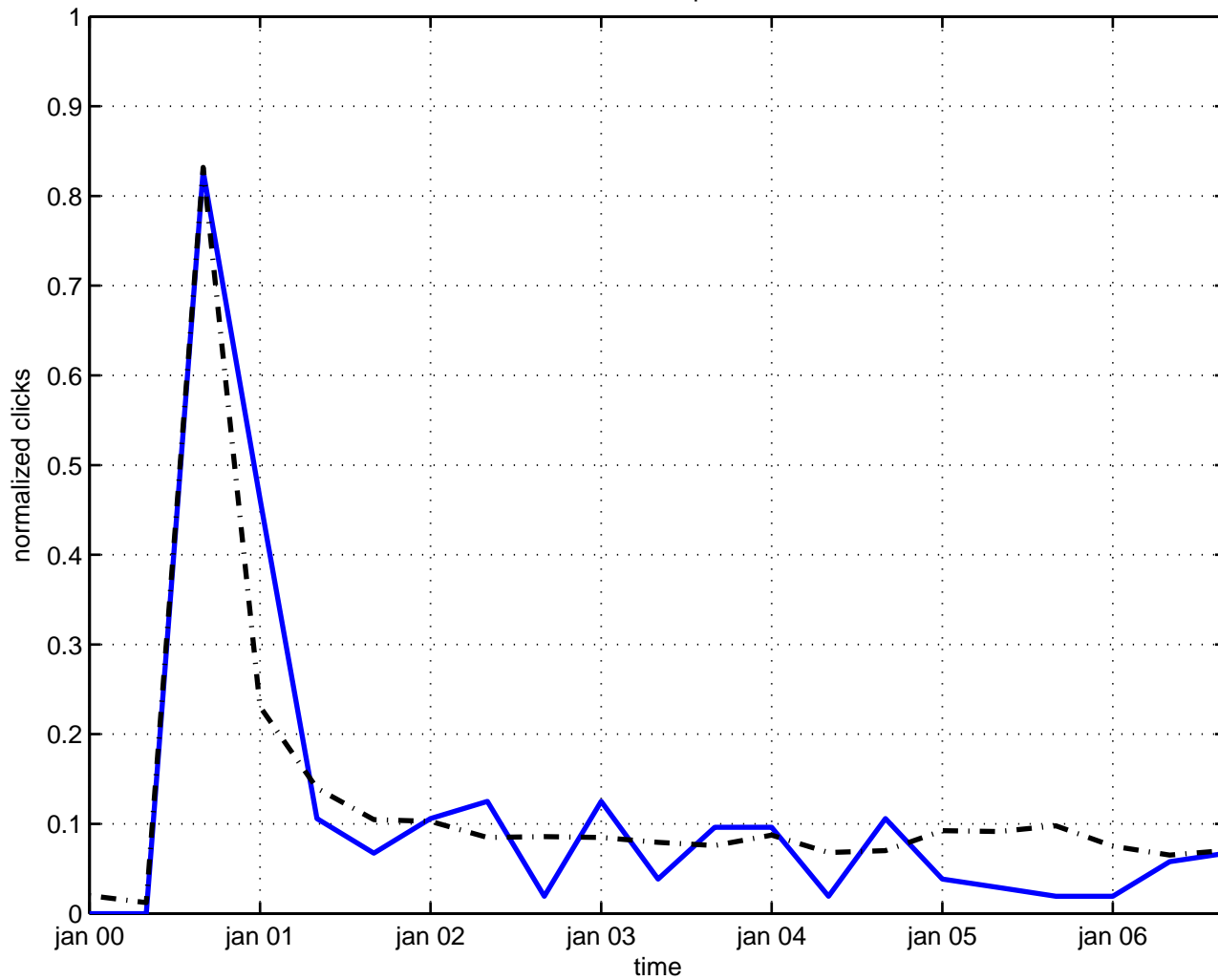
interaction d-particle
