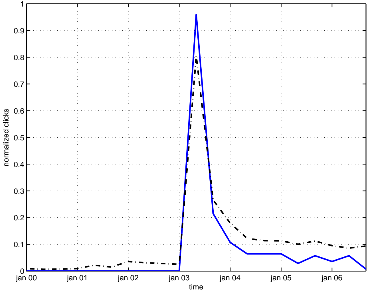
interaction d-brane
