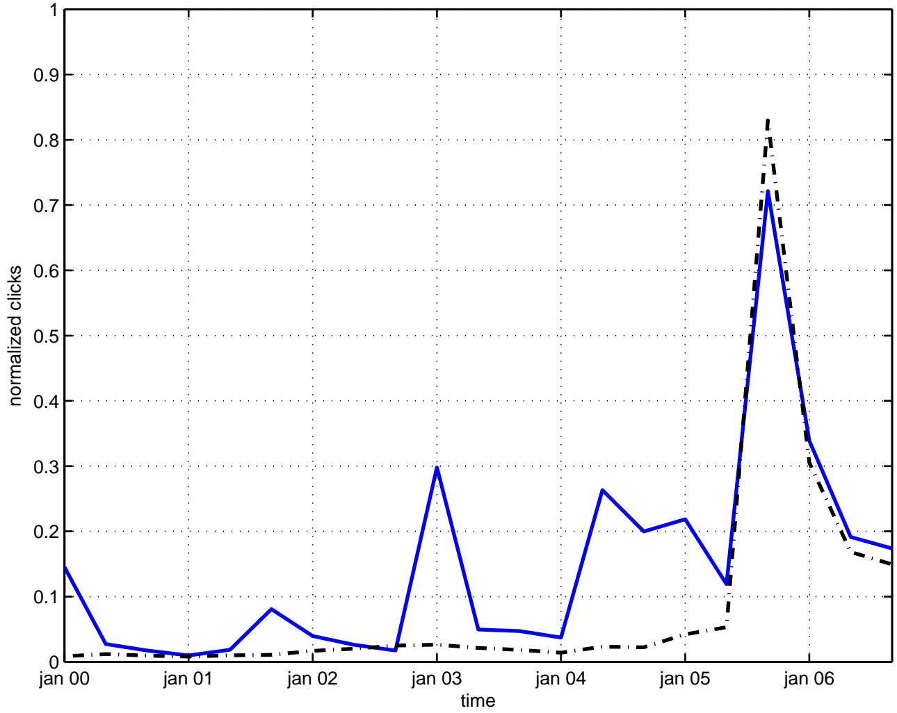
integral equations
