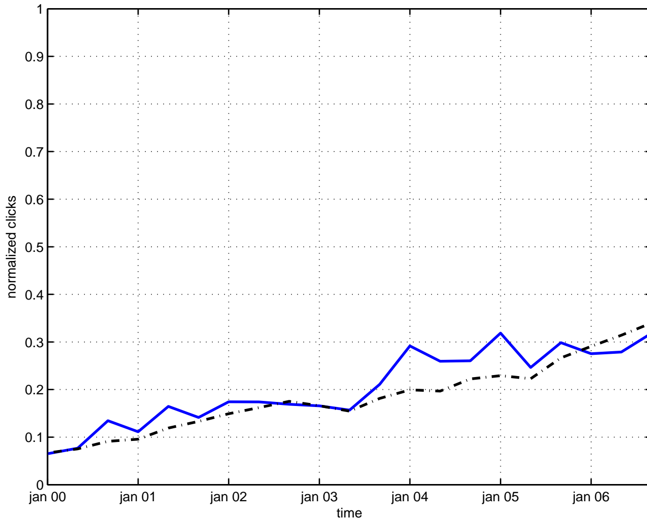
instanton
