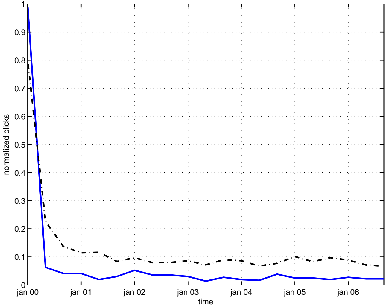
instanton membrane model
