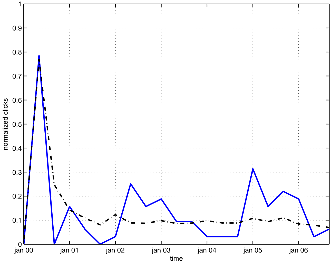
instanton approximation
