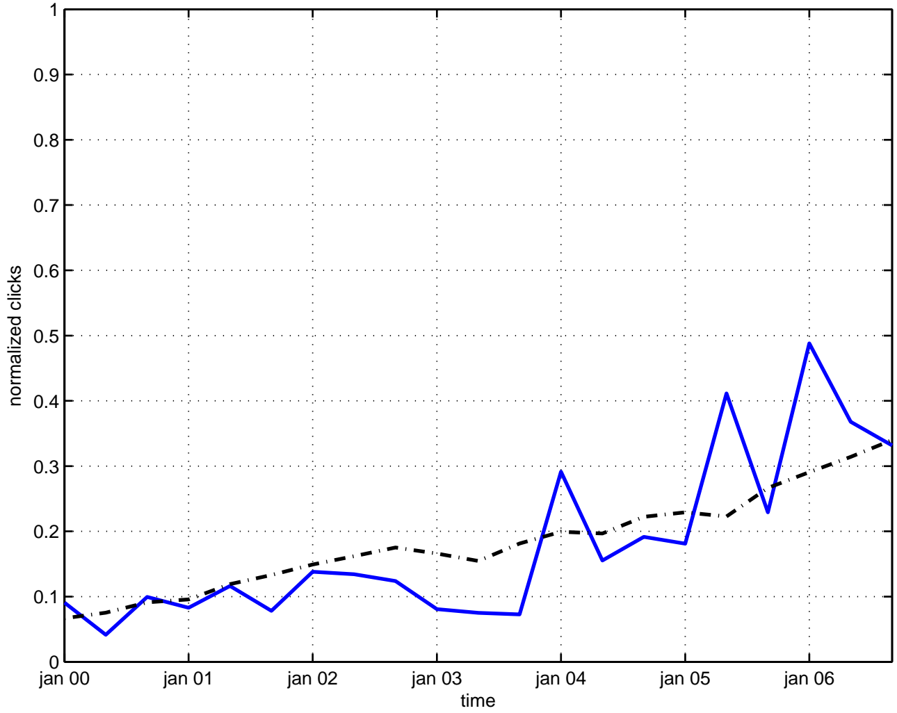
information theory
