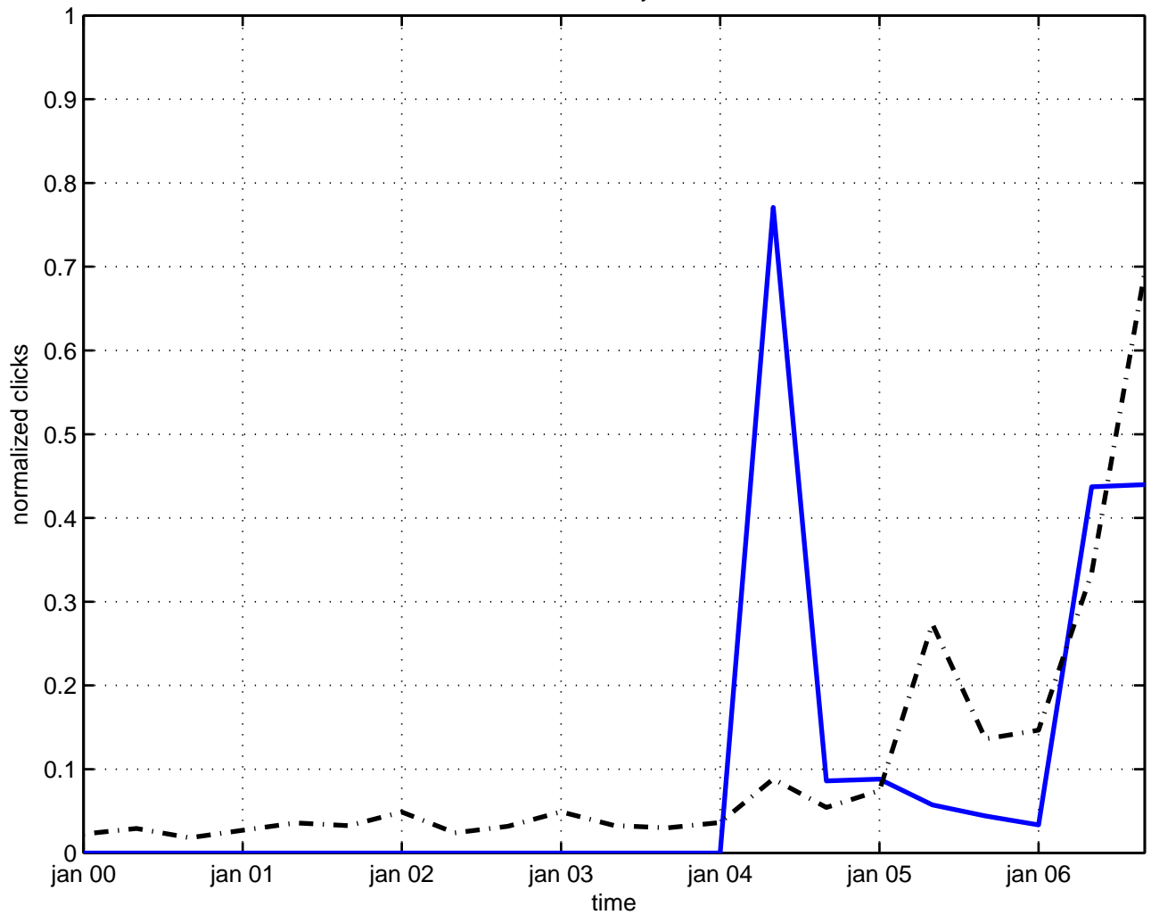
information theory black hole
