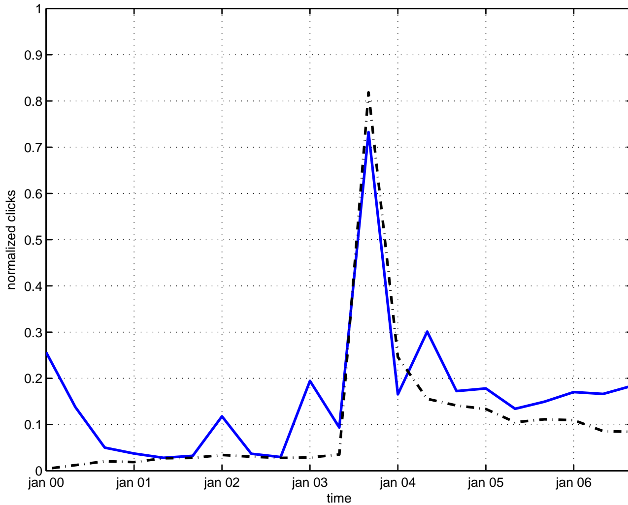
inflaton
