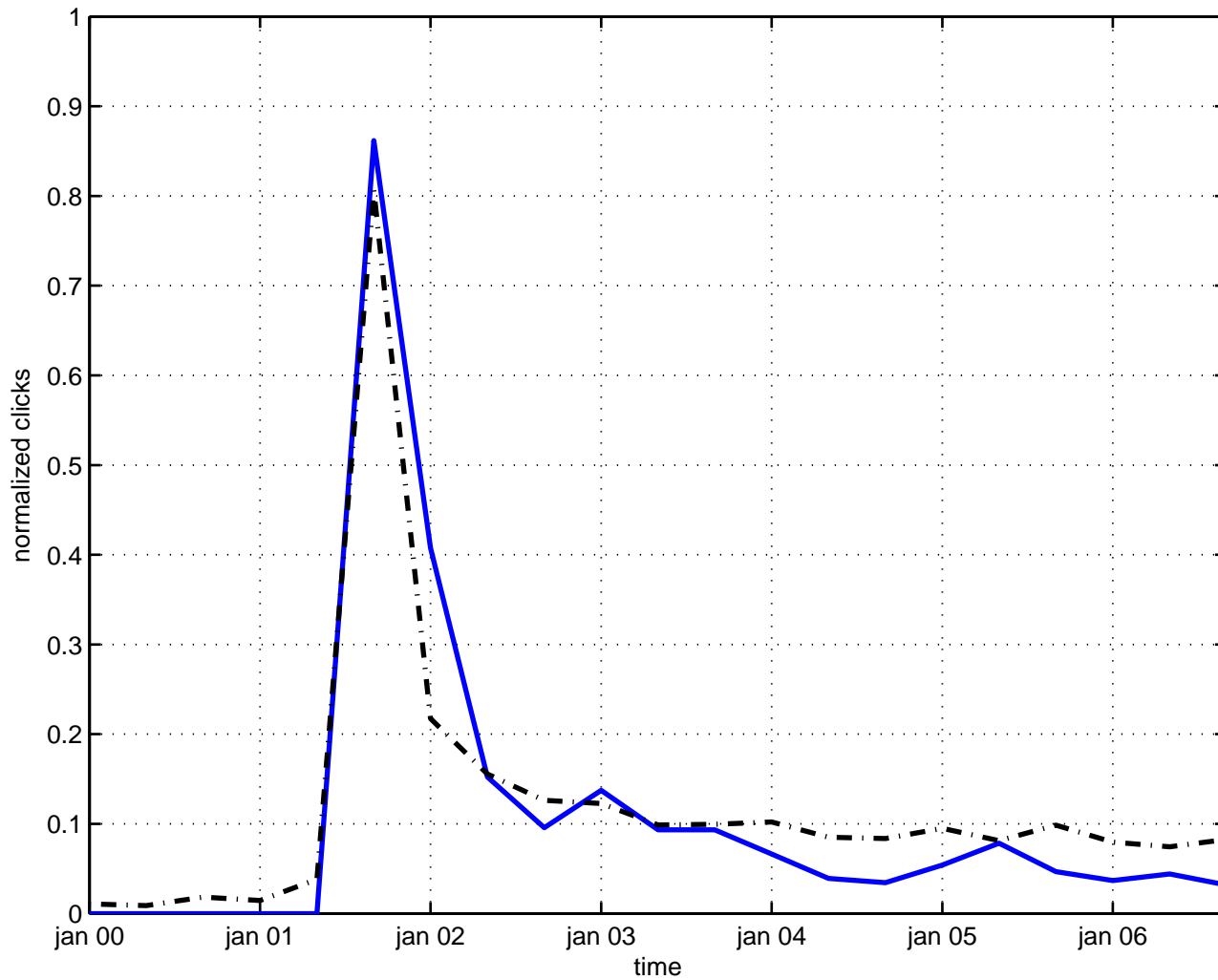
inflaton radion
