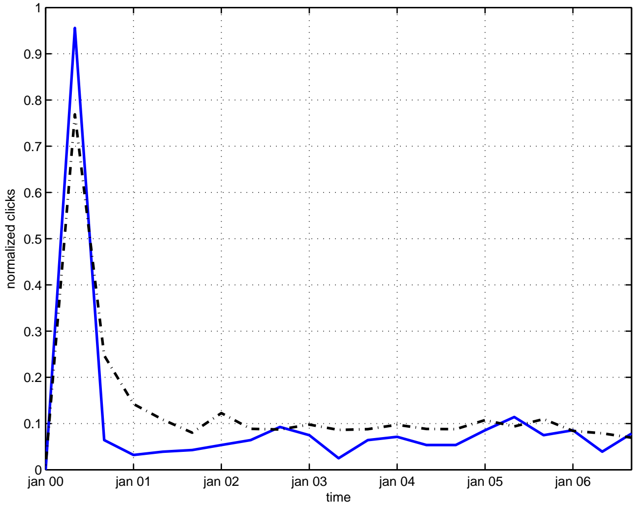
infinite statistics
