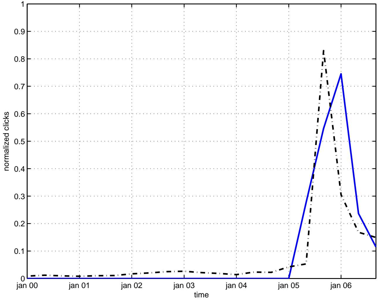
infinite dimension
