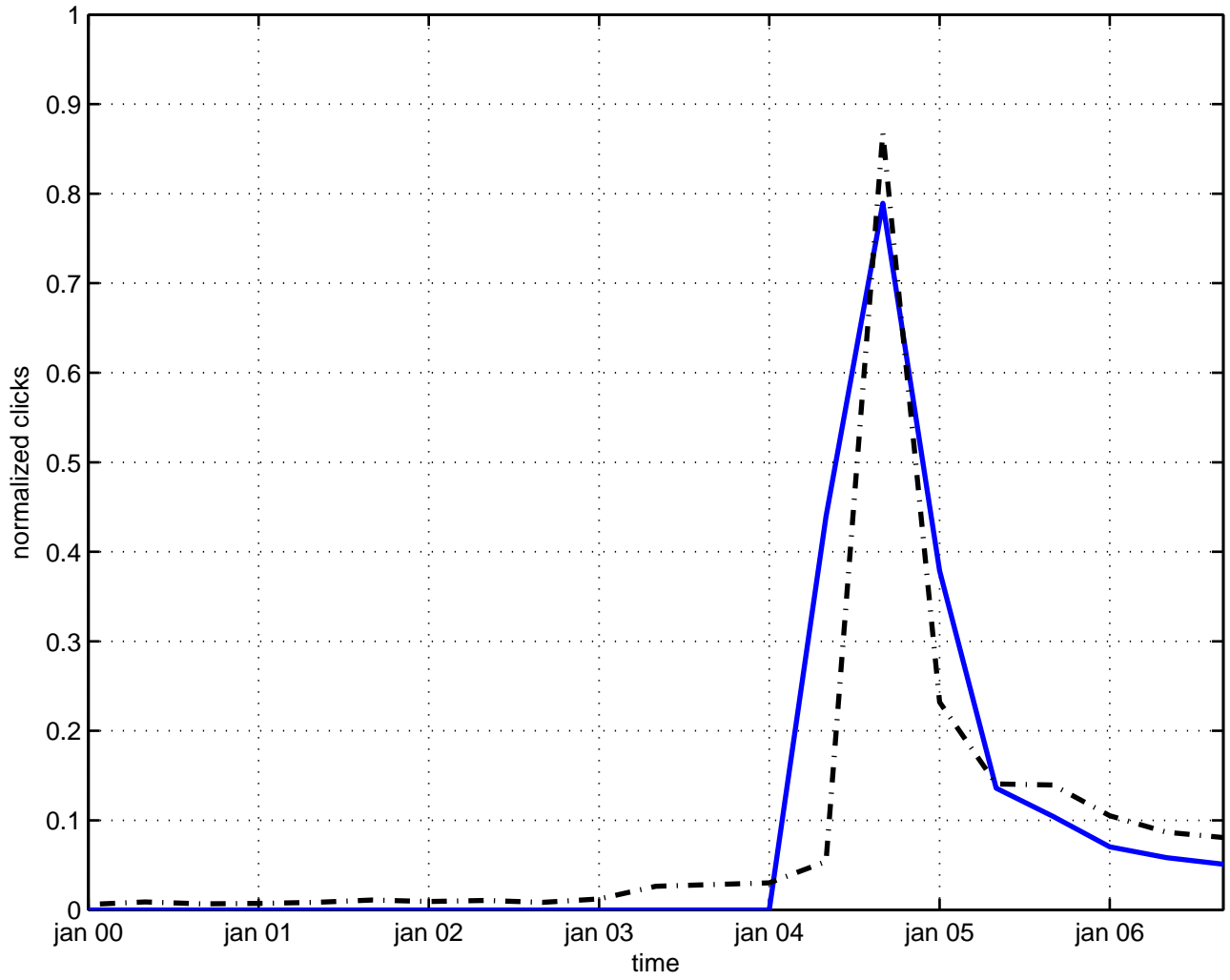
inelastic scattering
