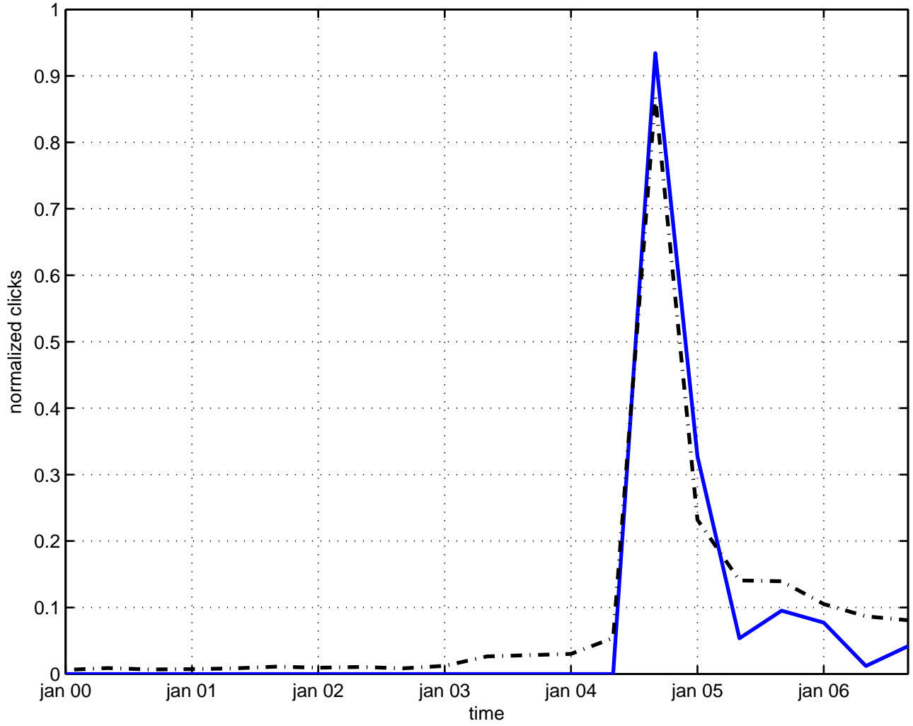
induced tunneling
