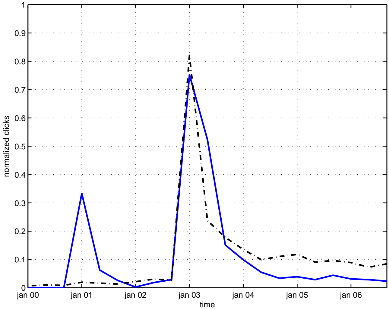
induced space-time
