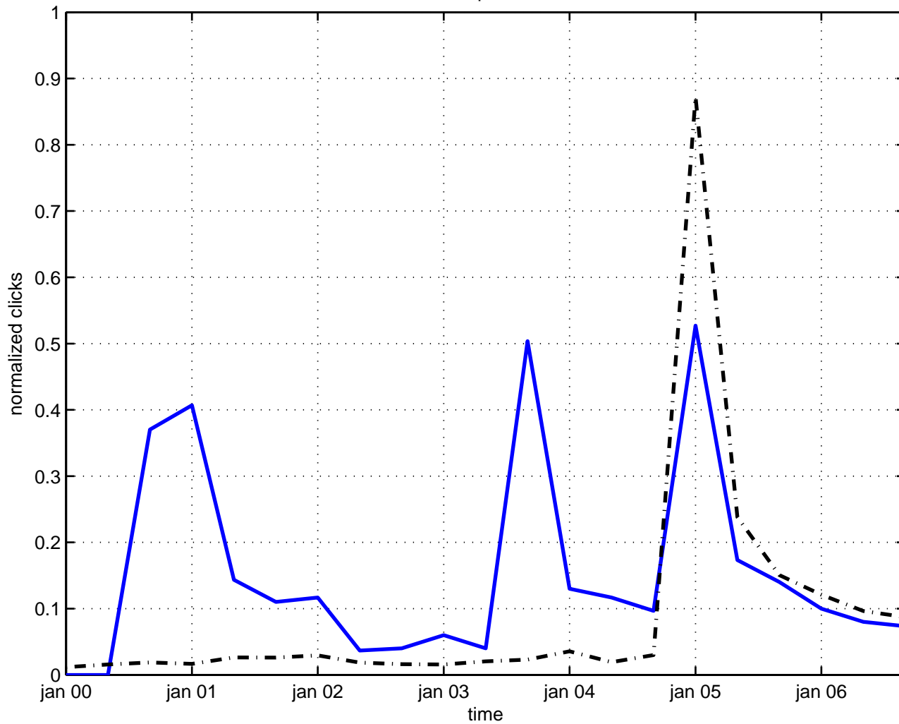
induced representation
