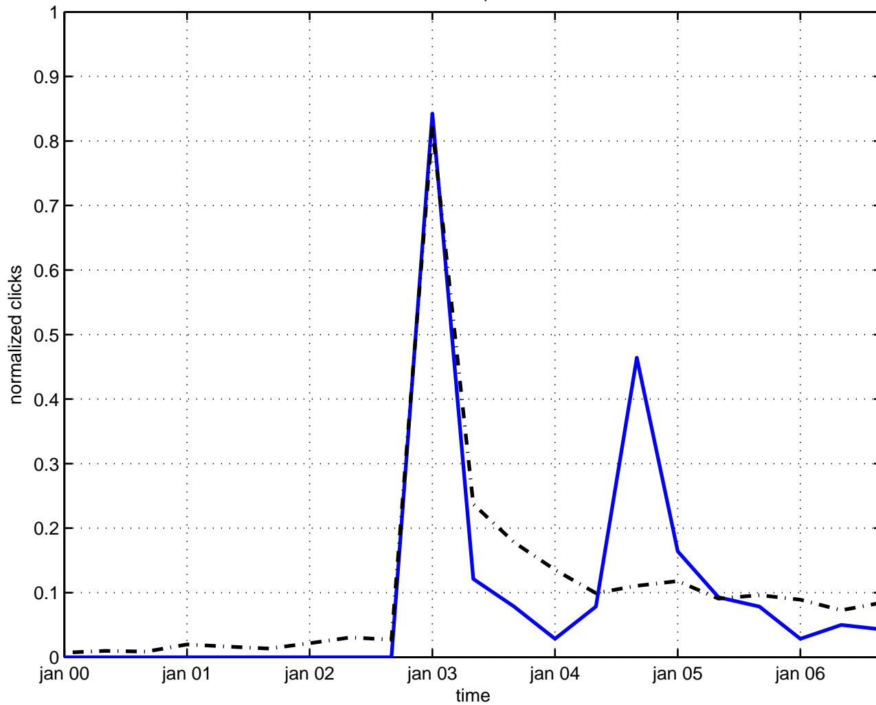
induced operator
