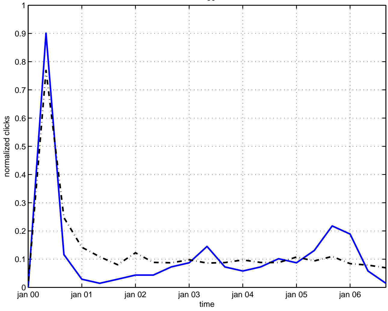
induced higgs model
