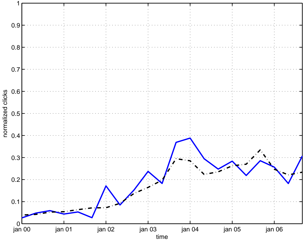
induced gravitation
