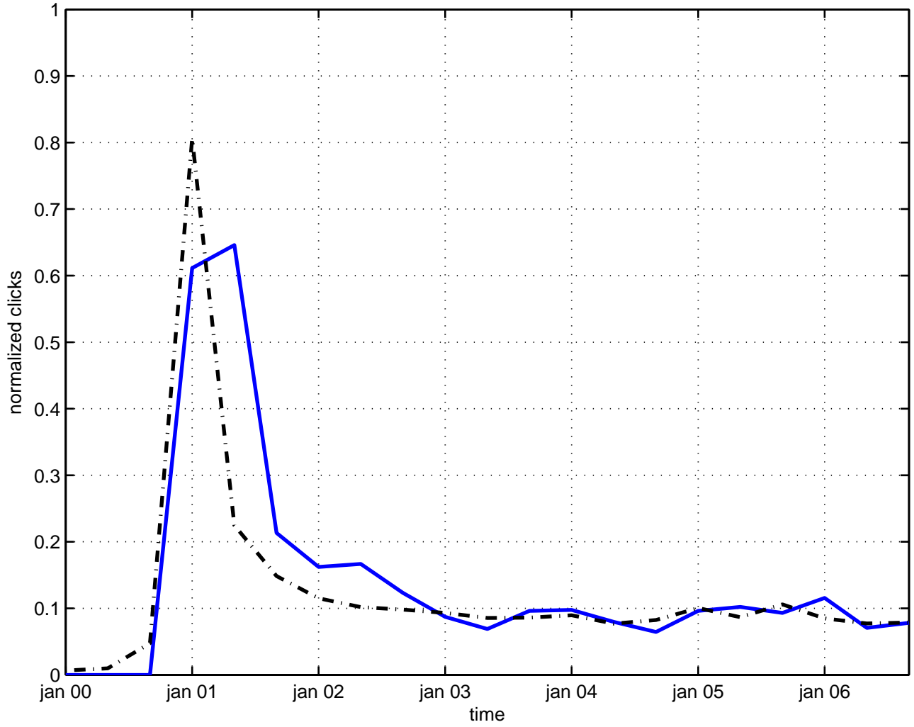
induced geometry
