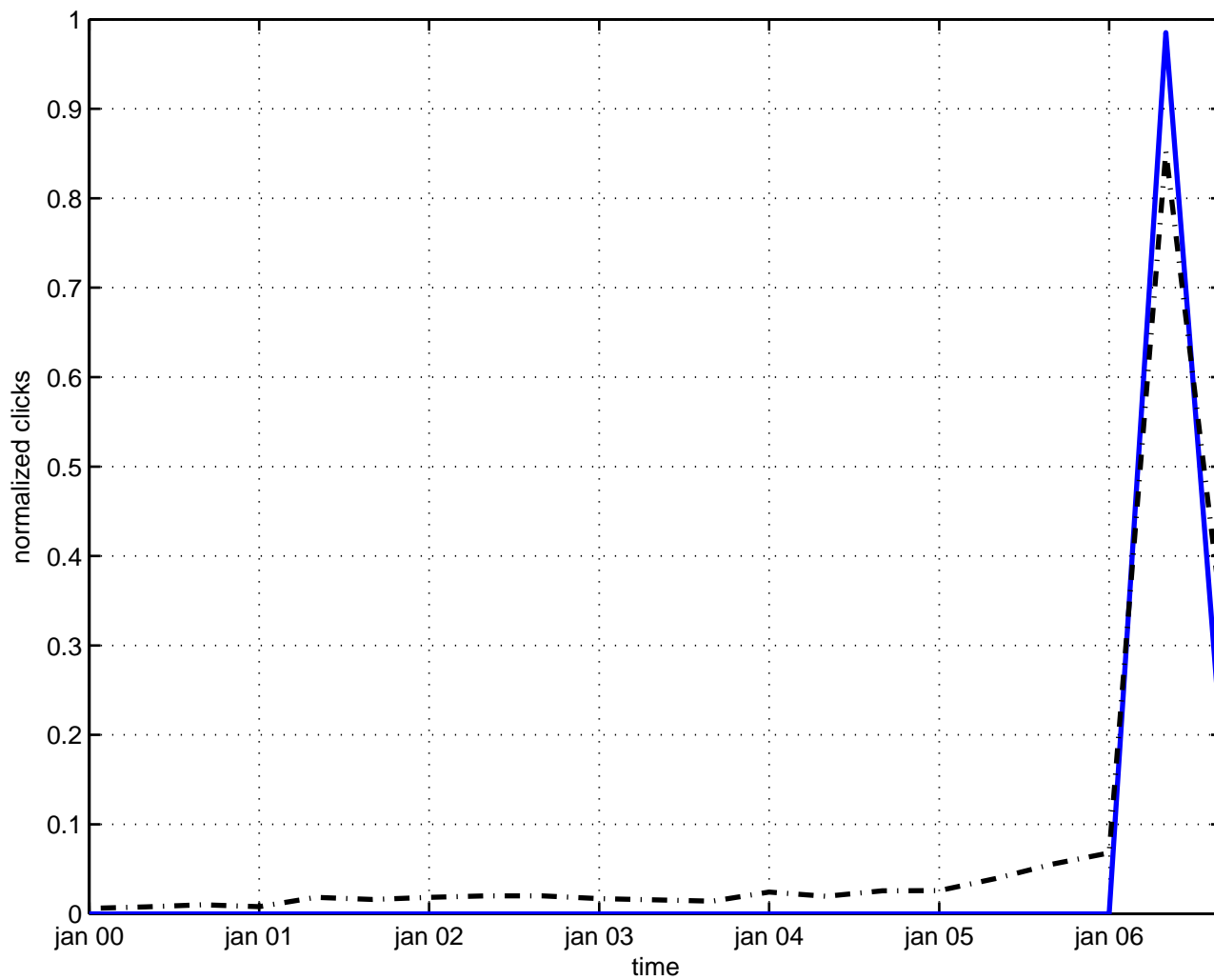
induced decoherence
