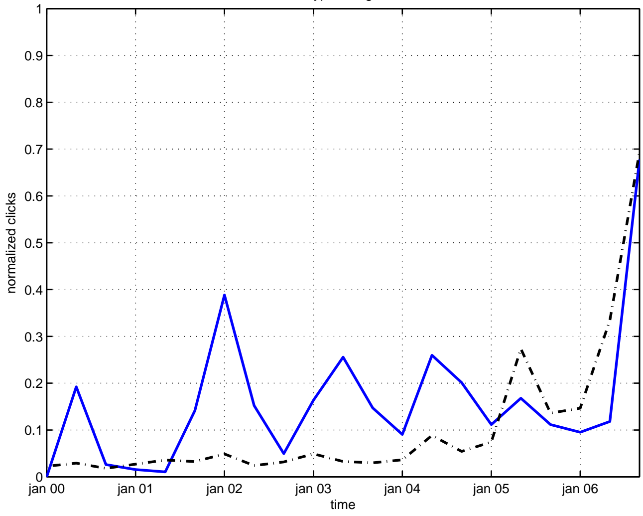
hypercharge
