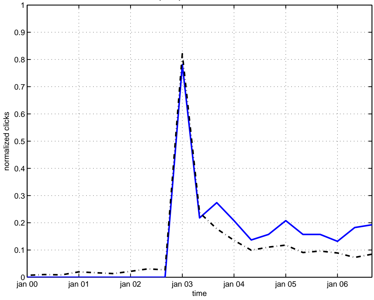
hydrodynamics fluctuation
