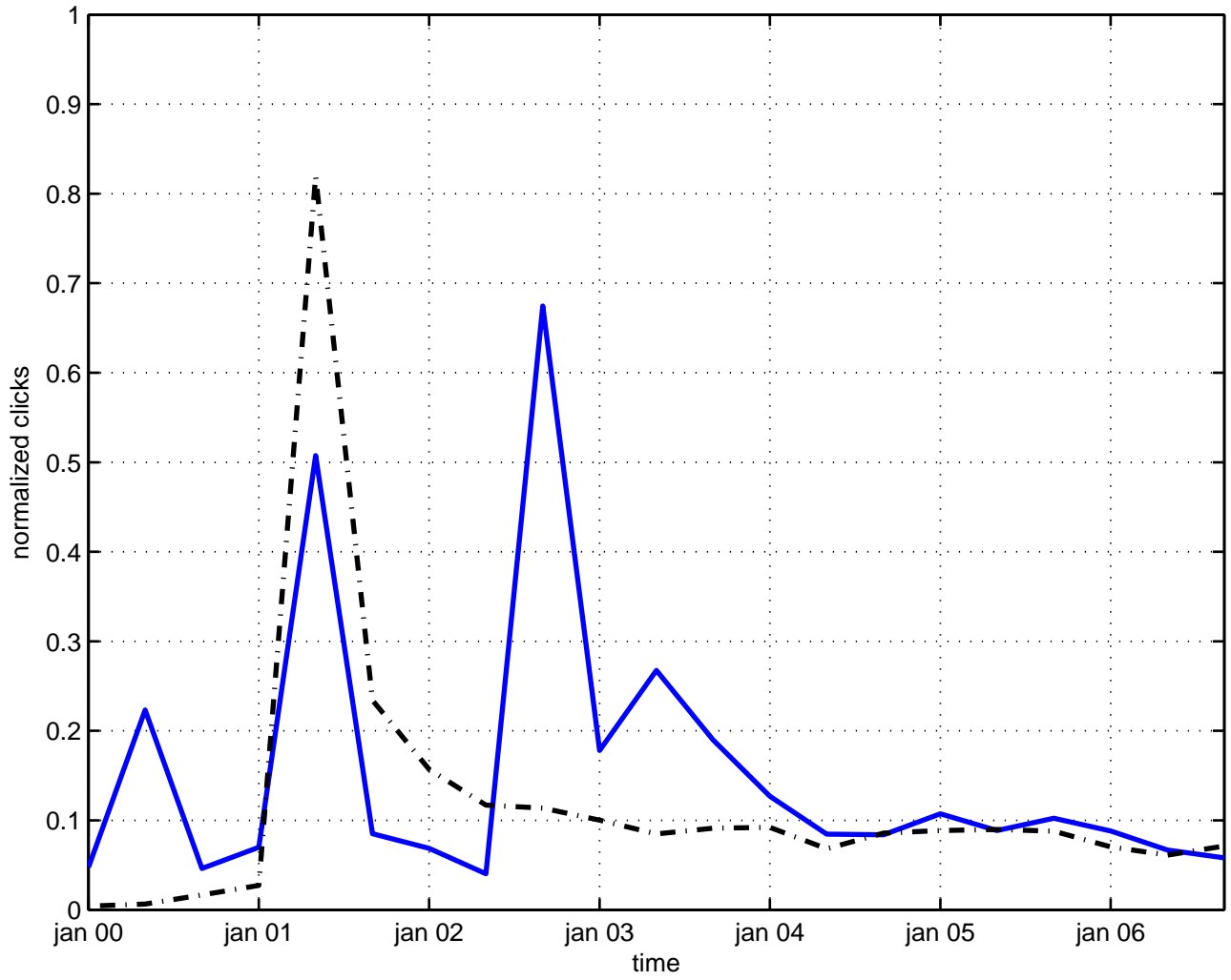
horizon space-time
