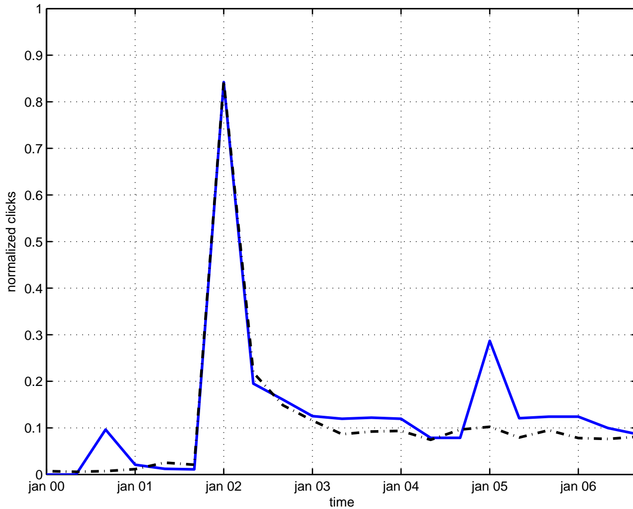
horawa-witten model
