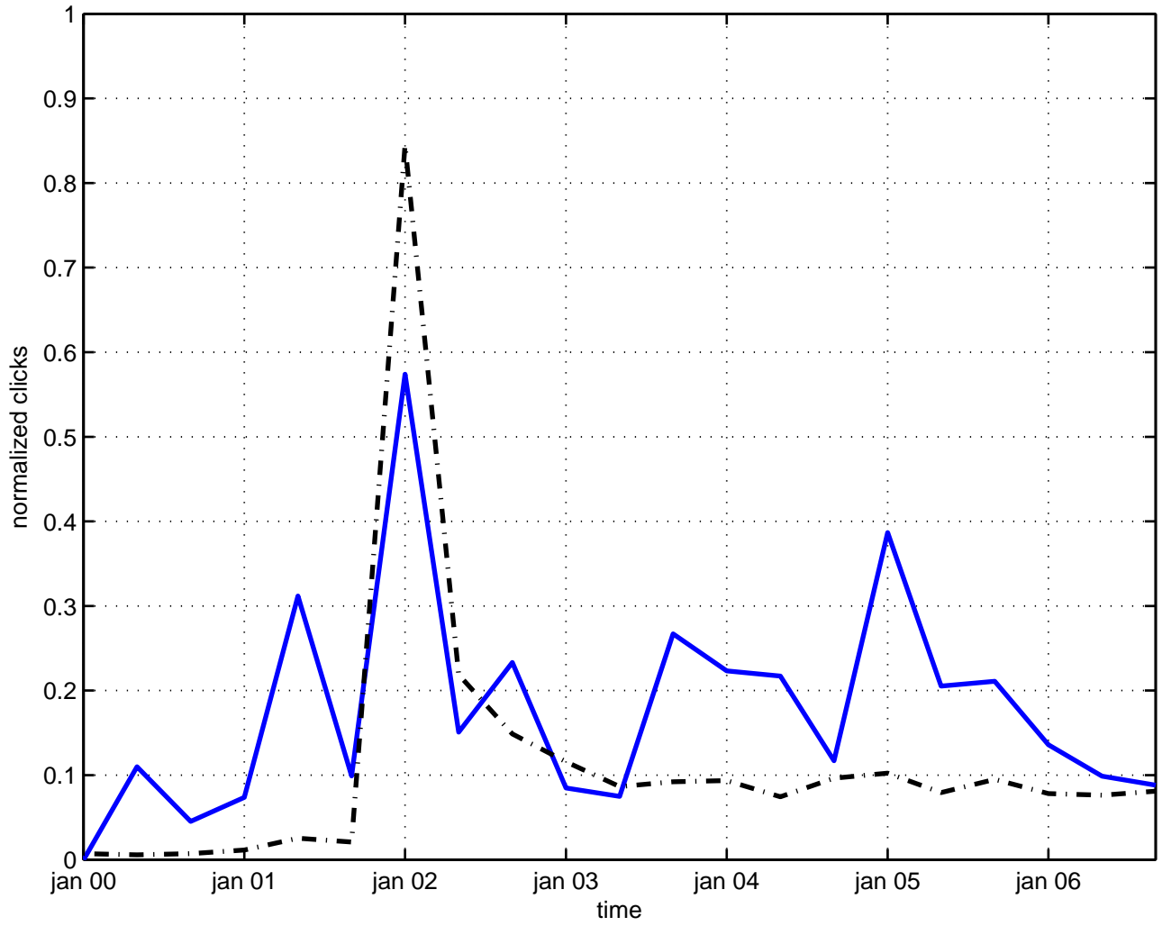
horava-witten model
