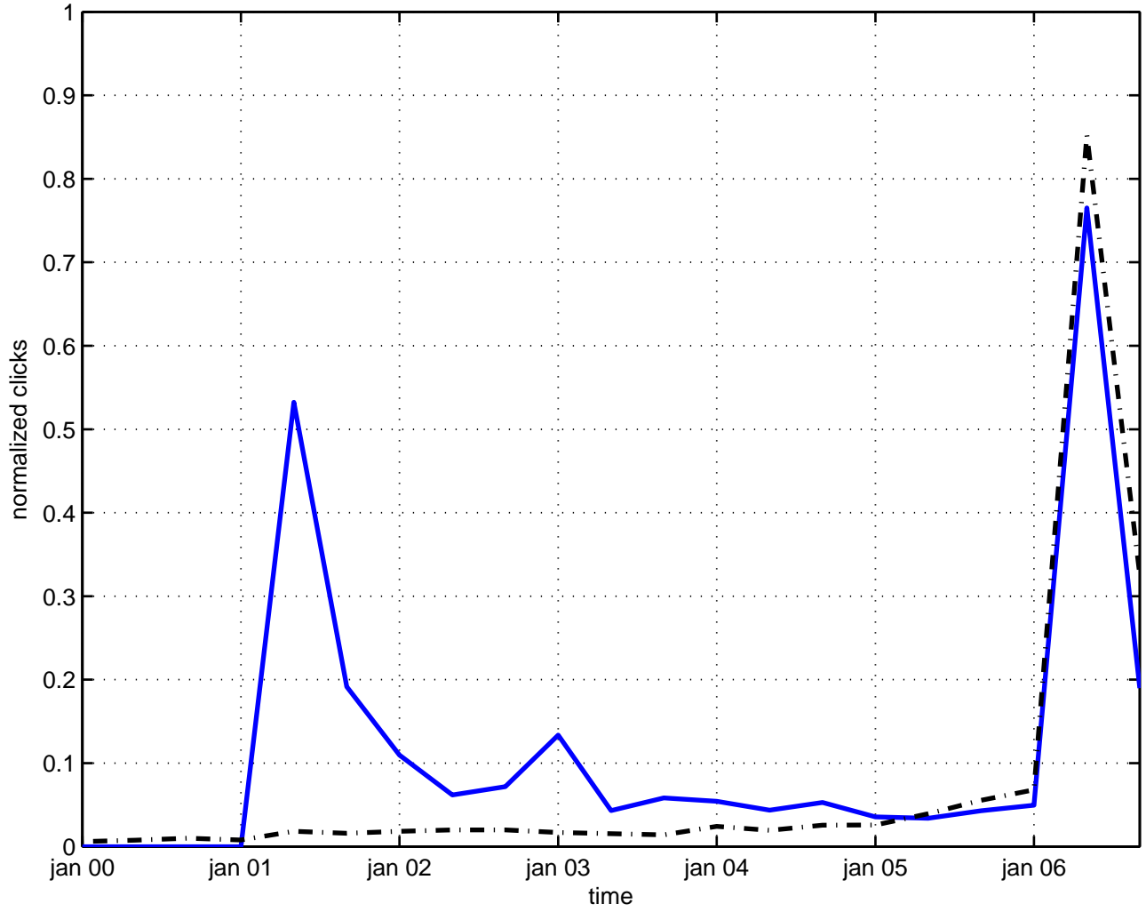
holography duality
