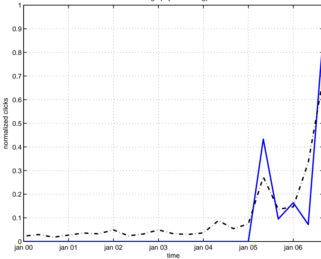
holography dark energy
