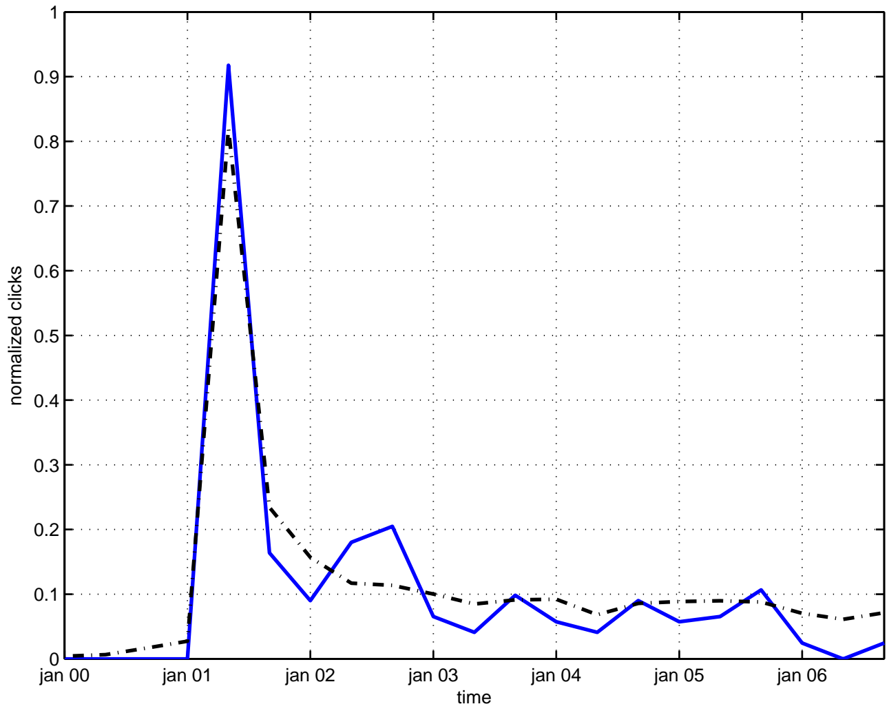
hofstadter model
