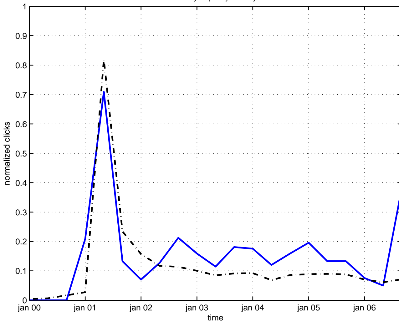
history supersymmetry
