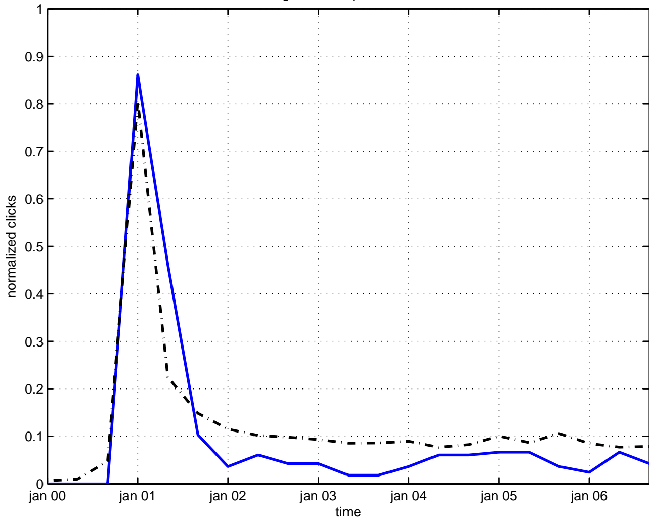
higher-order perturbation
