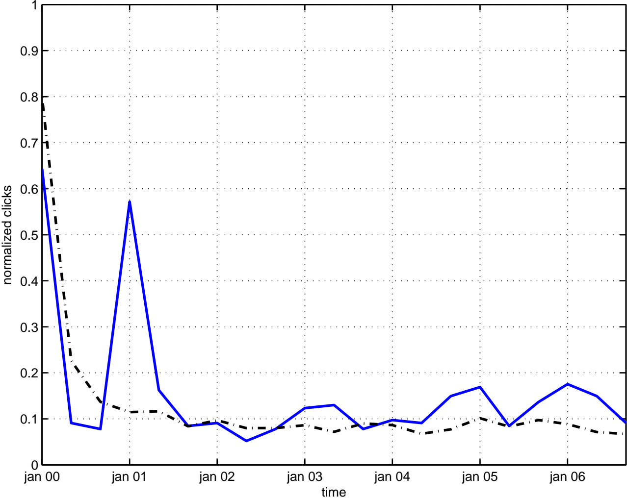
higher-order action
