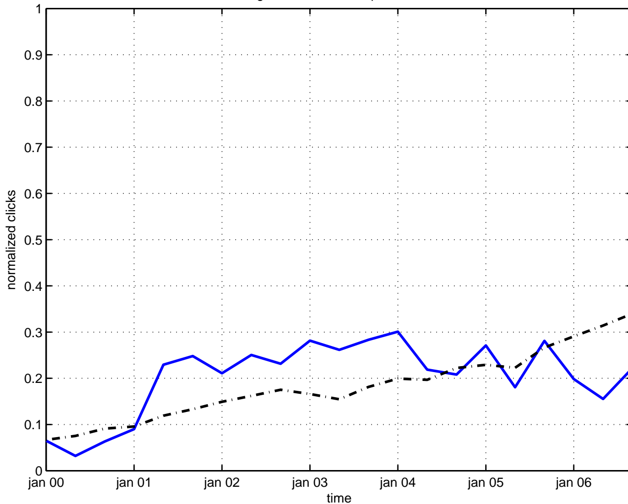
higher-dimensional space-time
