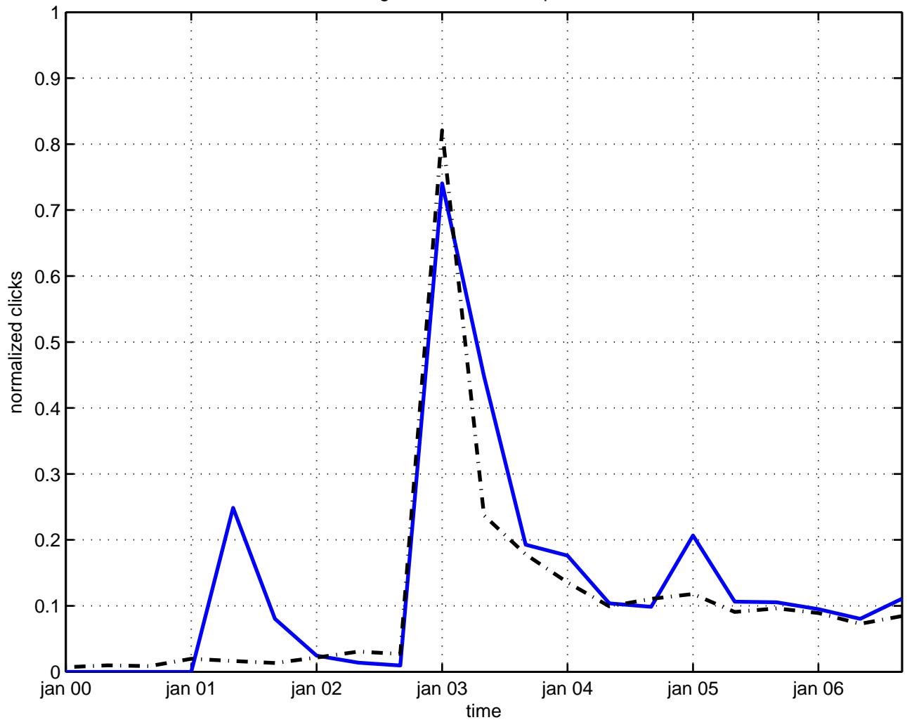
higher-dimensional operator
