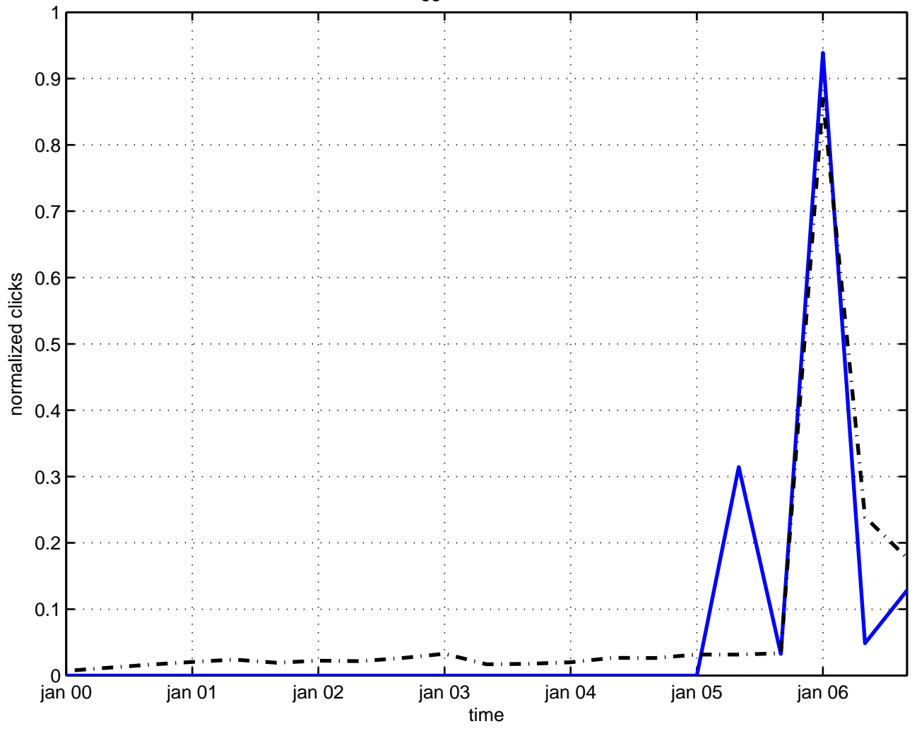
higgs-kibble model
