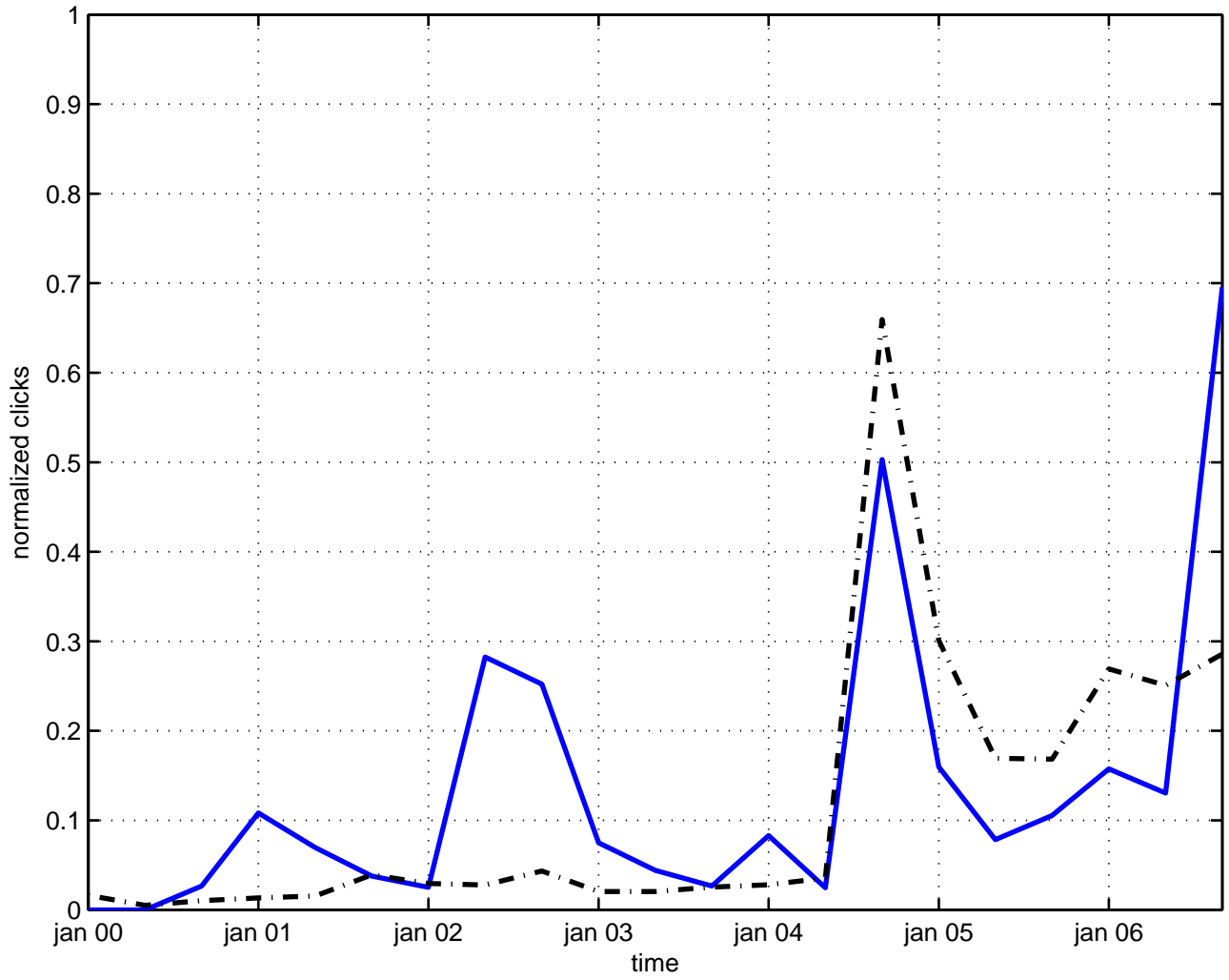
higgs particle
