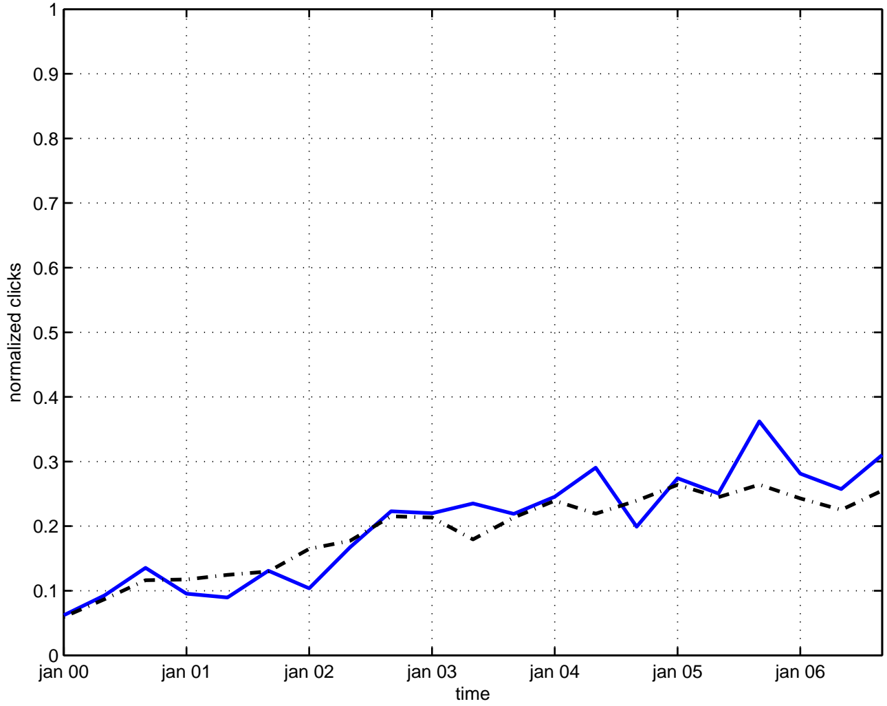
higgs model
