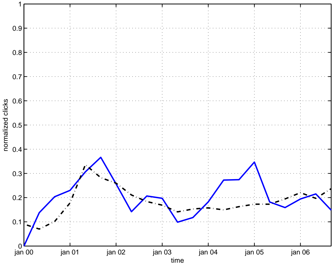
higgs mechanism
