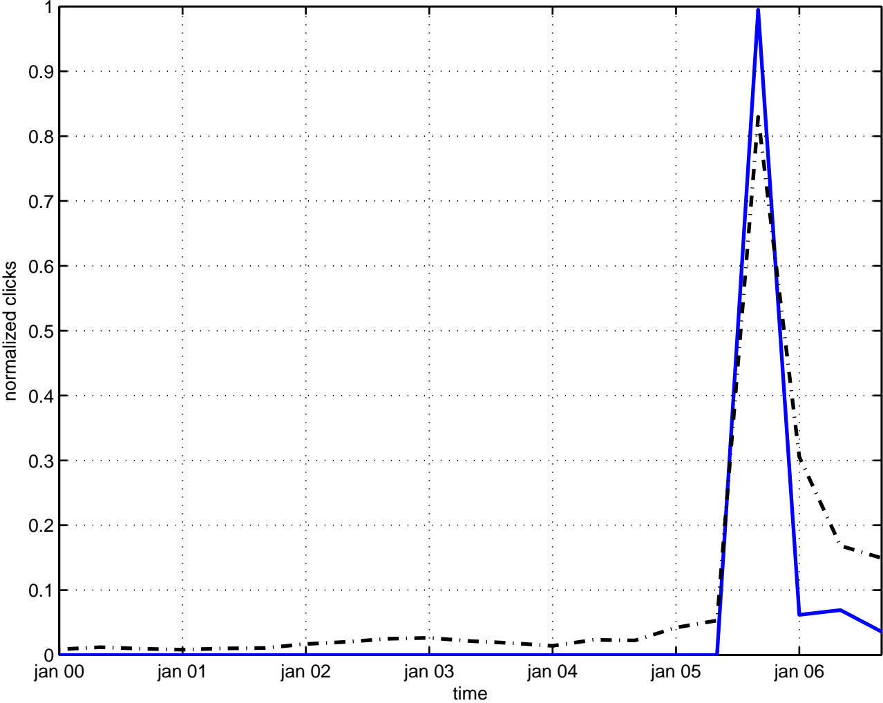
hierarchy gauge field theory
