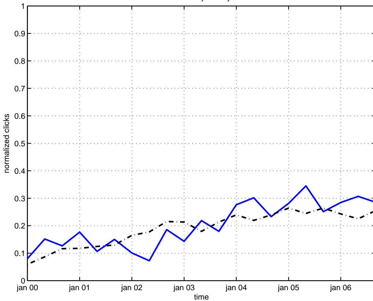
hidden symmetry
