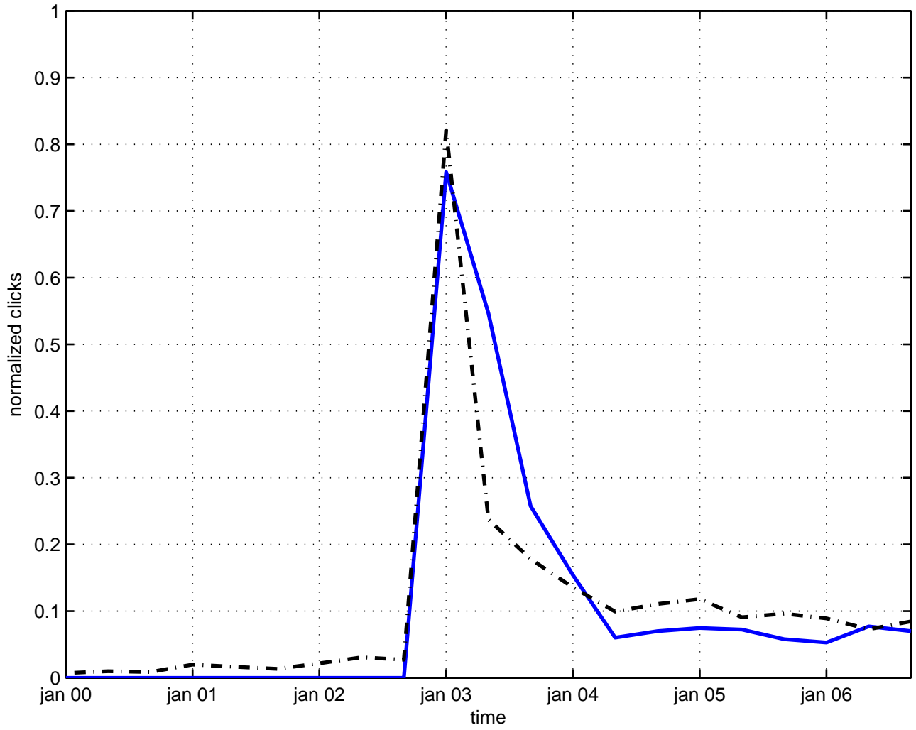
hidden symmetry space-time
