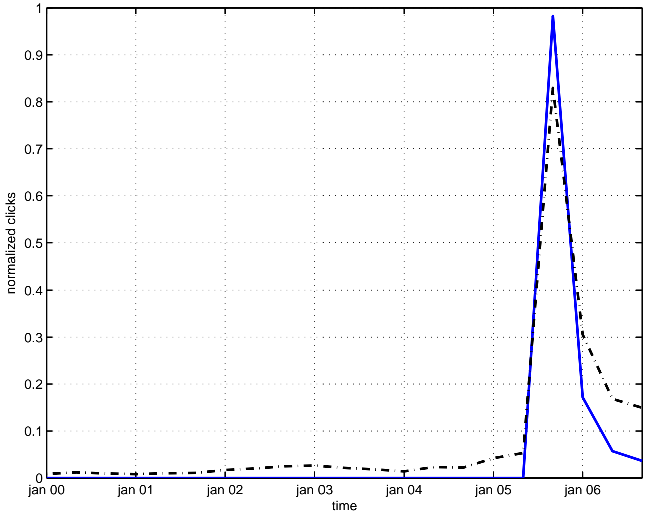
heterotic standard model
