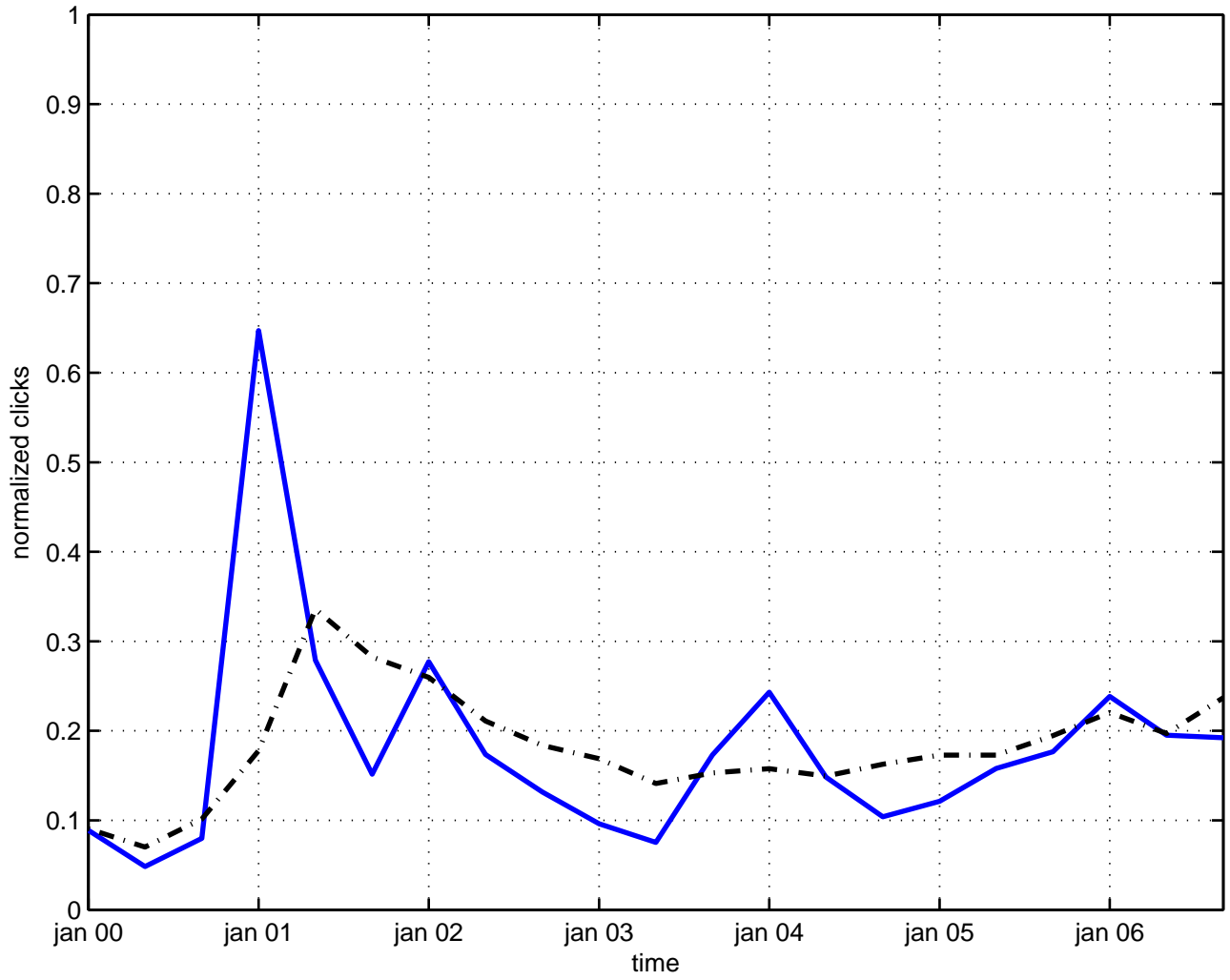
heterotic m-theory
