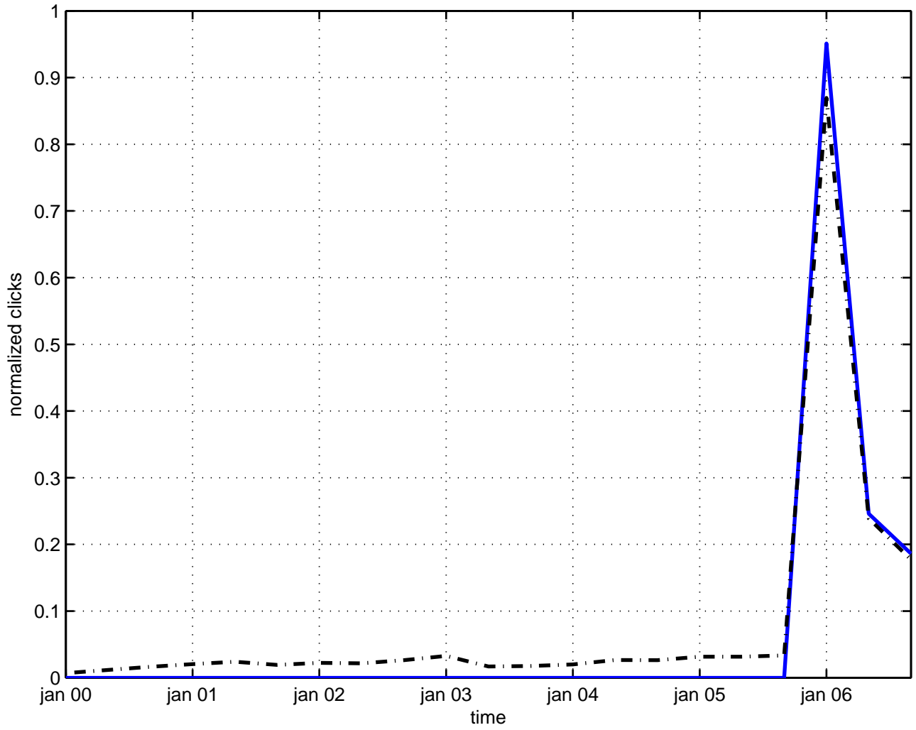
heterotic flux
